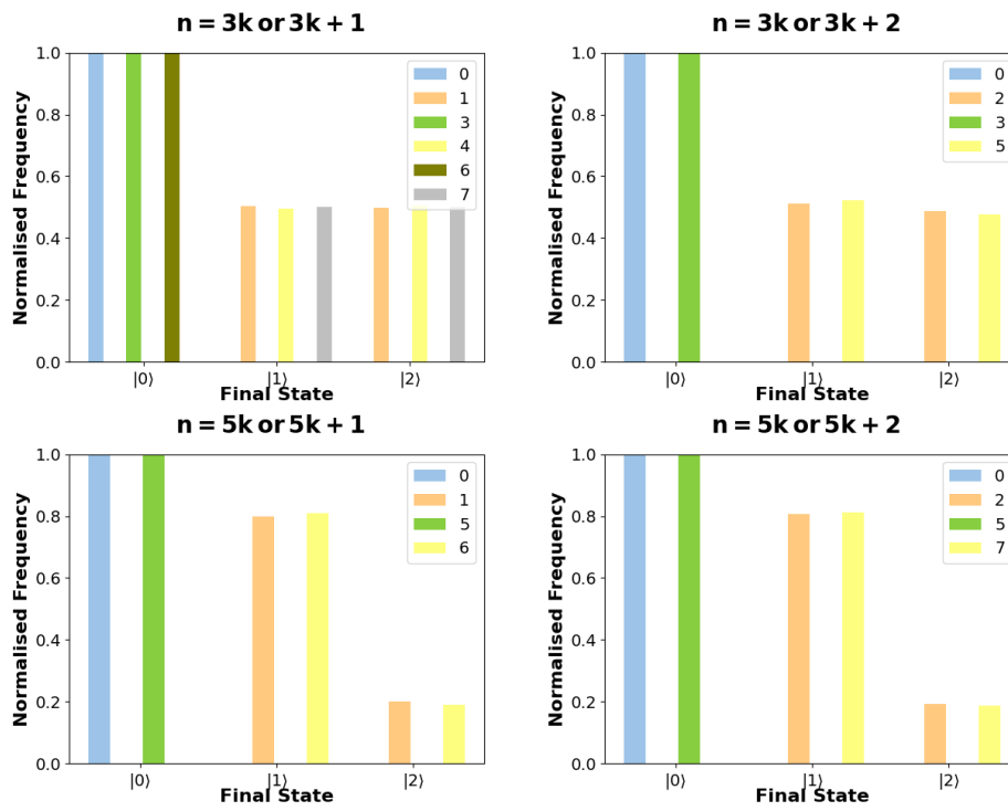
Figure 5.4: Results of Running Tian et al. (2019) on an IBM Qiskit Simulator
