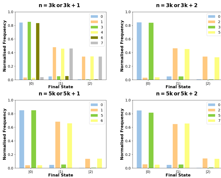
Figure 5.5: Experimental Results of Running Tian et al. (2019) on IBM Qiskit Hardware
